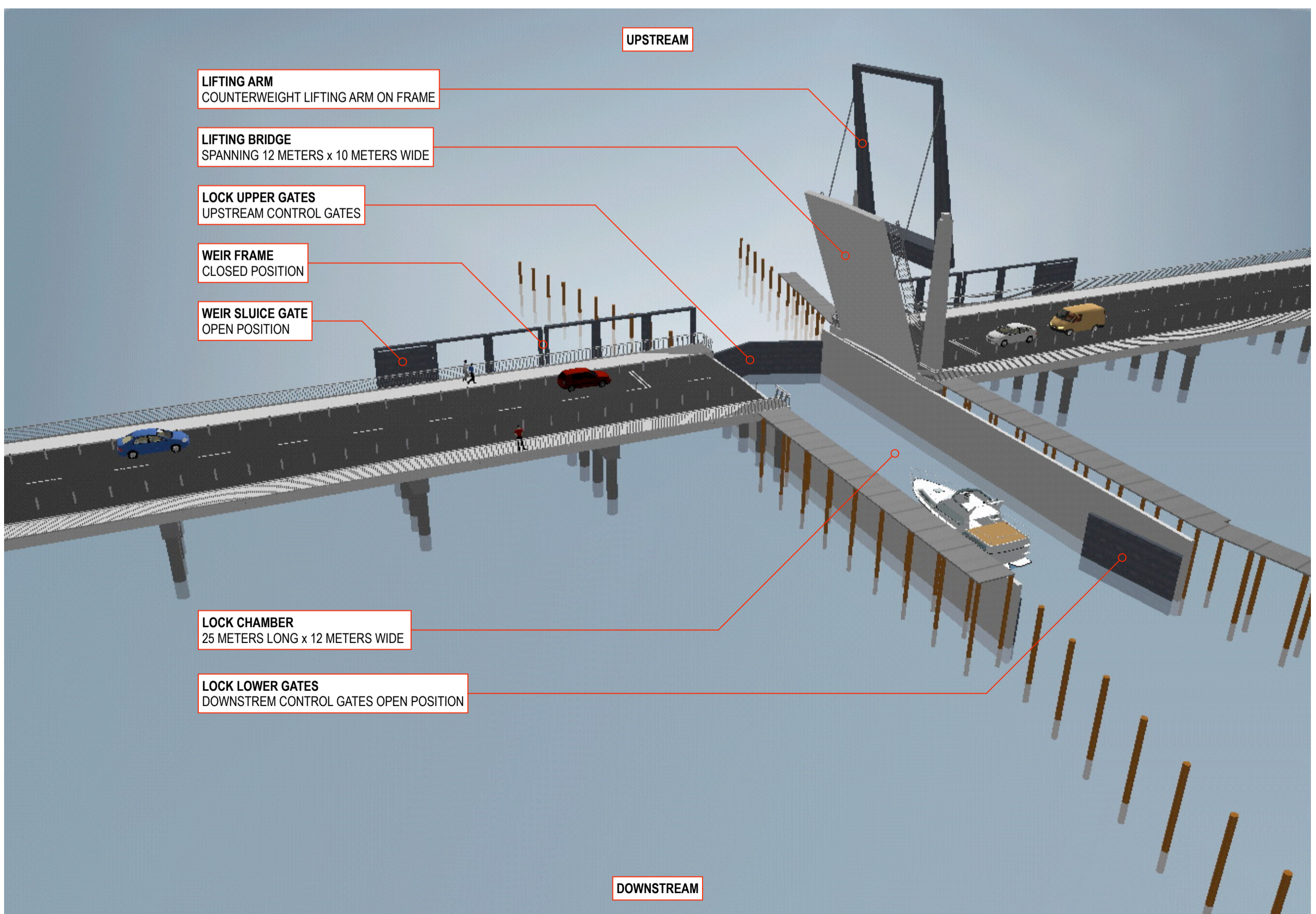
LOCK OPTION
