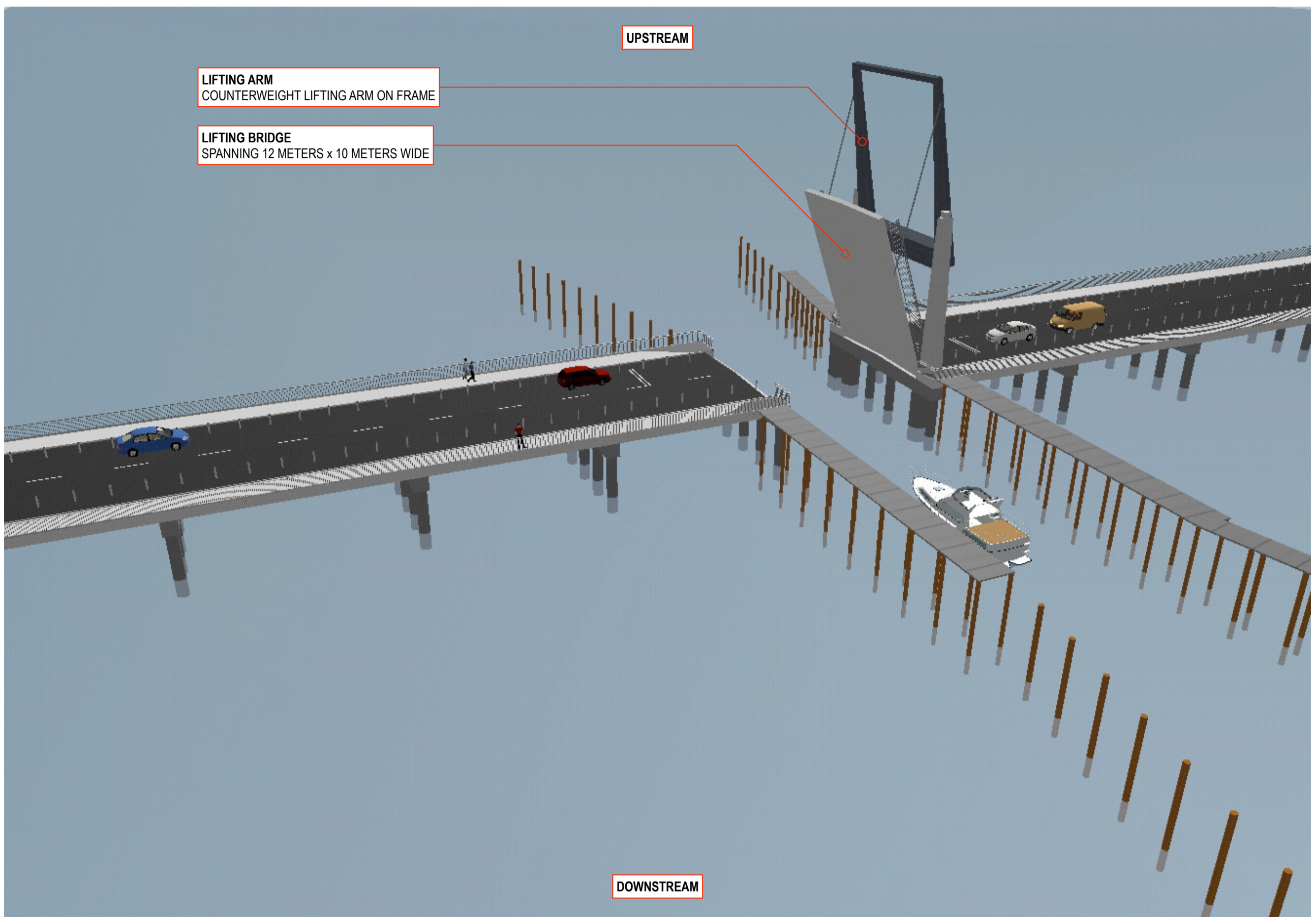
BRIDGE OPTION
